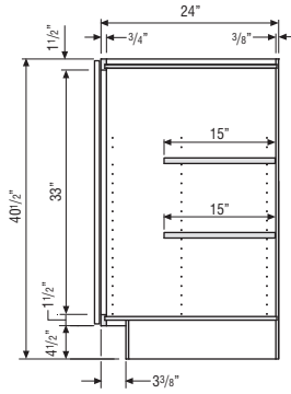
40 1/2" HIGH FULL HEIGHT BASE CABINET
