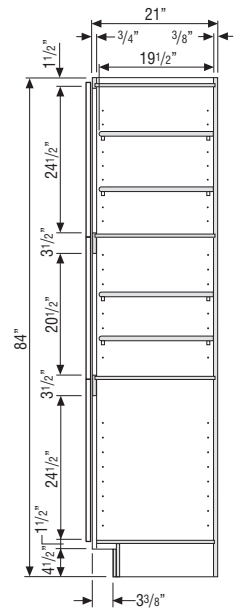
VANITY UTILITY CABINET
