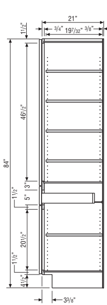
LINEN TALL with DRAWER
