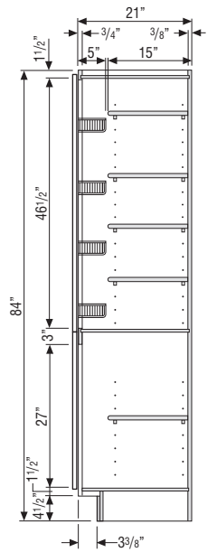
LC/LCRH/LT CABINET
