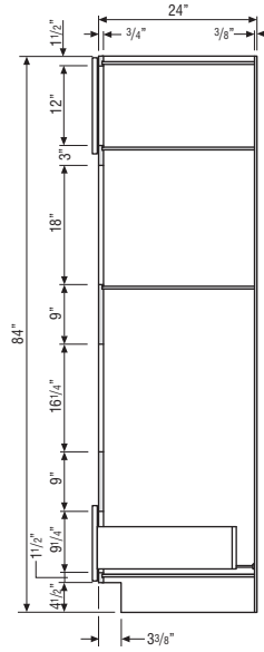
OVEN MICROWAVE CABINET DEEP DRAWER
