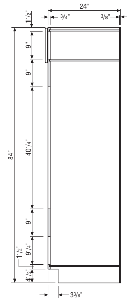
DOUBLE OVEN CABINET WARMING DRAWER with EXTENDED OPENING
