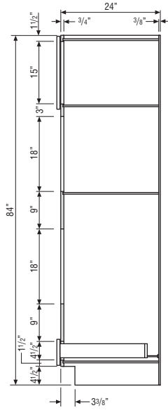
OVEN MICROWAVE CABINET
