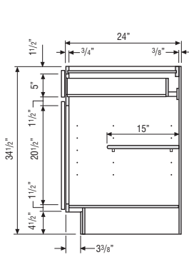
BASE CABINET
