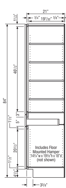
LINEN TALL with DRAWER and REMOVABLE HAMPER
