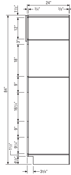
OVEN MICROWAVE CABINET WARMING DRAWER
