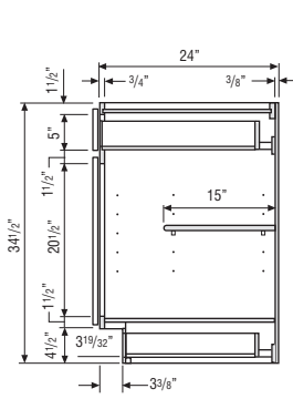
BASE CABINET with TOEKICK DRAWER
